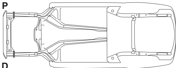
UNDERBODY VIEW
